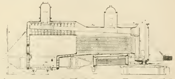
ROGERS' COAL BURNING BOILER. FIG. 67
